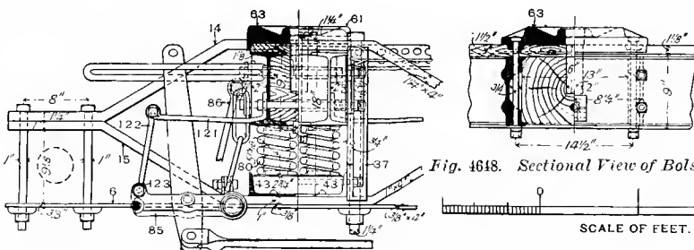
Fig. 4647. Half Longitudinal Section and Part Side Elevation. (With Malleable Iron Center-plate.)
